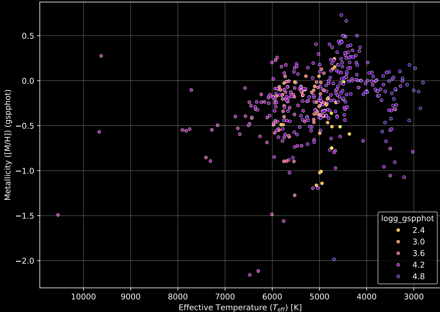
APOGEE DR17 Field: [221+84] Stellar Population Parameters (n= 416)
