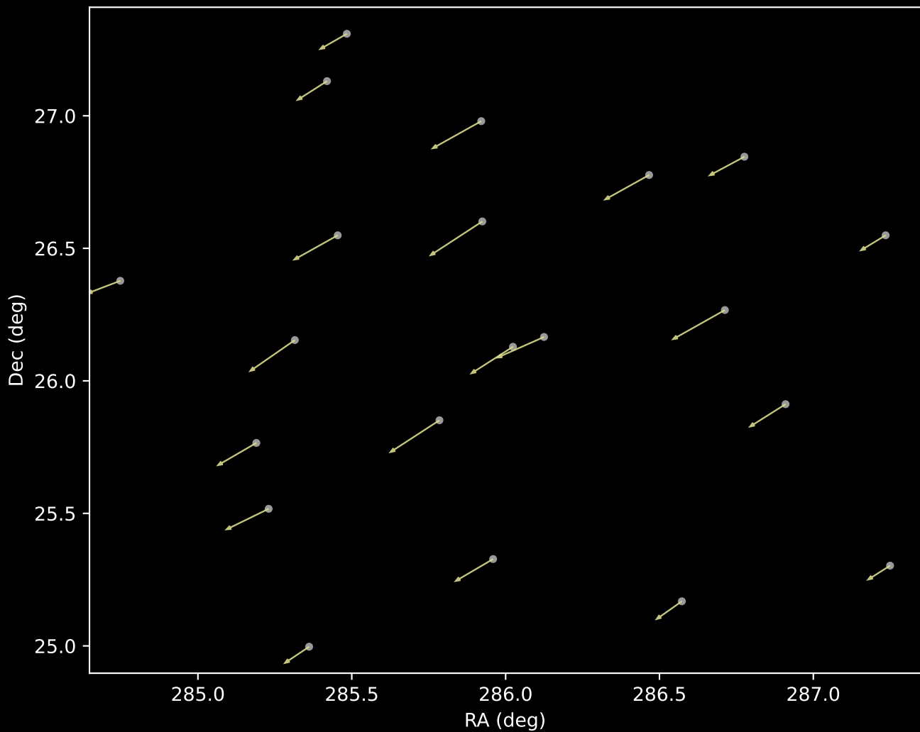
APOGEE DR17 Cluster 17 Proper Motion Vectors (n=21)
