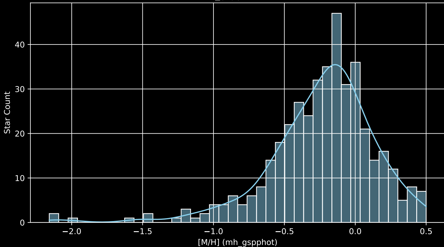
APOGEE DR17 Field: [221+84 [M/H] (mh_gspphot) (n= 414)
