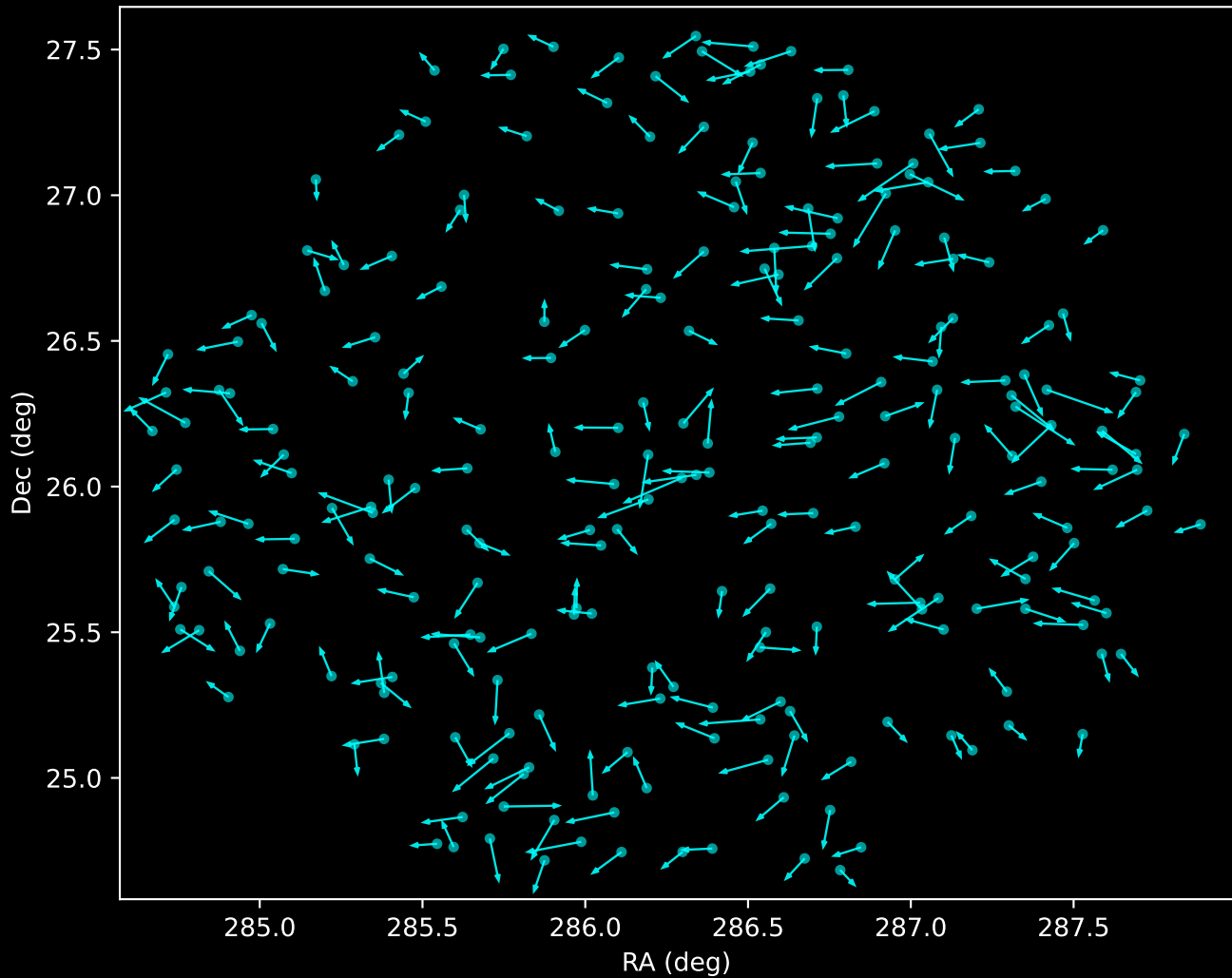
APOGEE DR17 Noise Stream Proper Motion Vectors (n=239)
