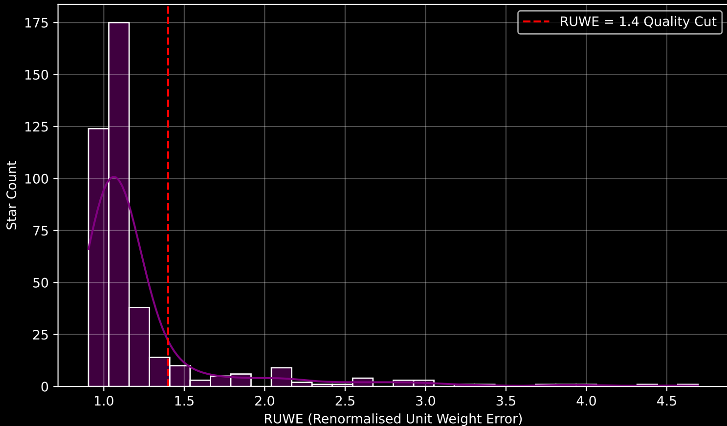
GAPOGEE DR17 Field [221+84] RUWE Distribution (n= 405)
