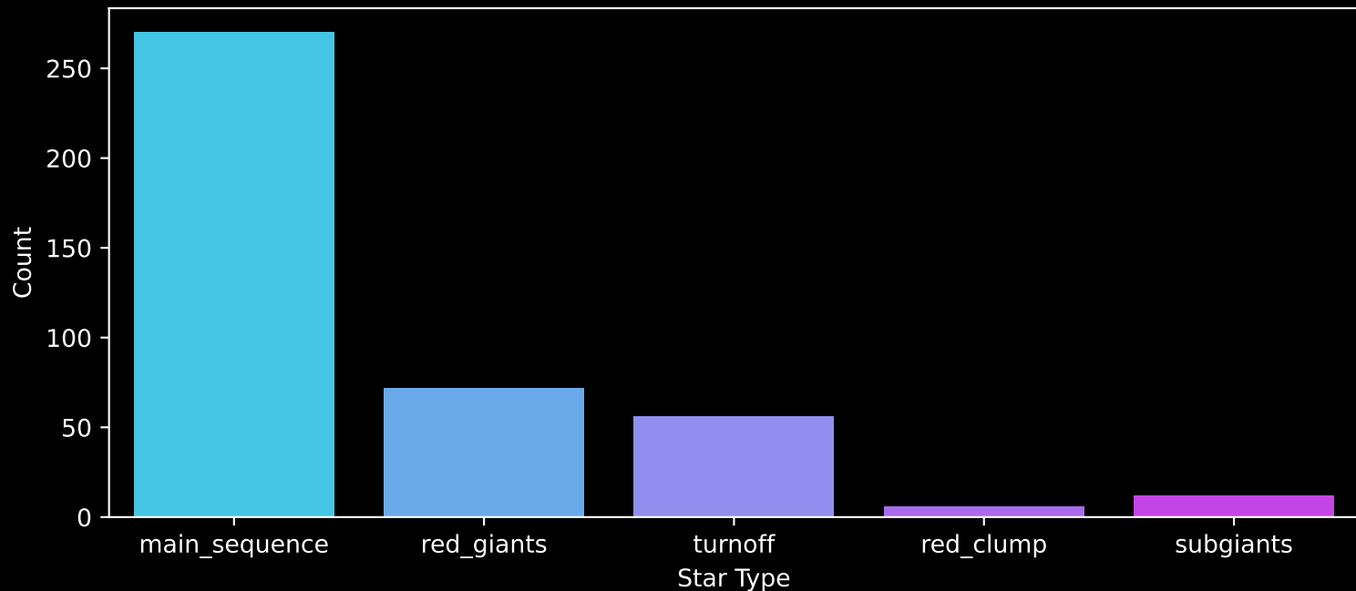
APOGEE DR17 Field: [221+84] Count plot of Star Type
