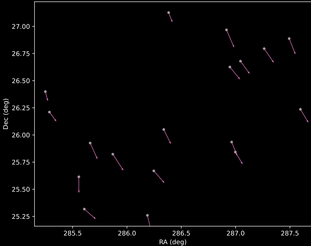
APOGEE DR17 Cluster 12 Proper Motion Vectors (n=18)
