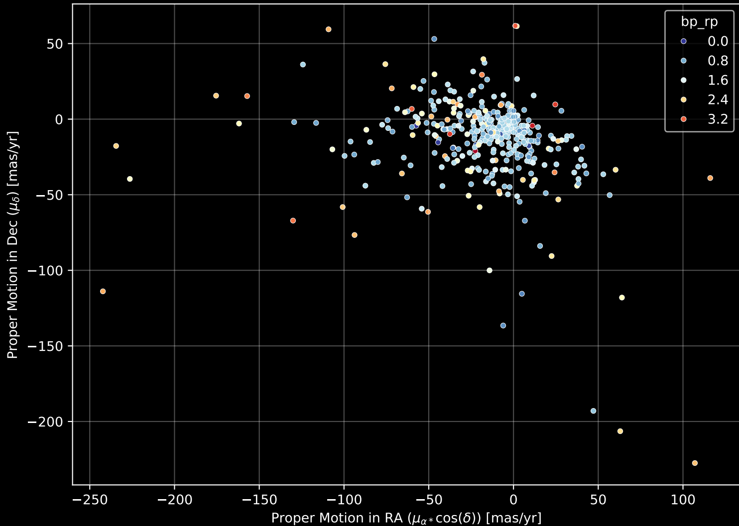
APOGEE DR17 Field: [221+84] Proper Motion Diagram (n= 416)
