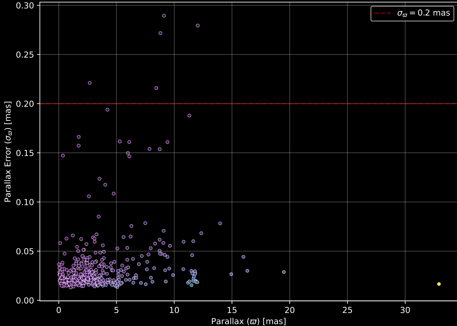
APOGEE DR17 Field: [221+84] Parallax Quality (n= 416)
