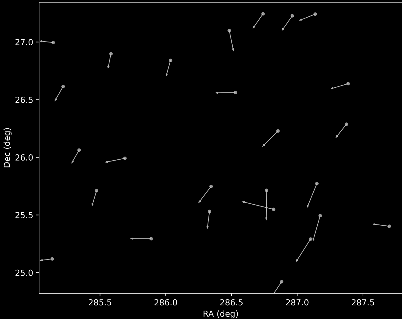
APOGEE DR17 Cluster 15 Proper Motion Vectors (n=26)
